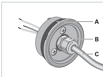
Fig. 8: Luminaire RL70.
