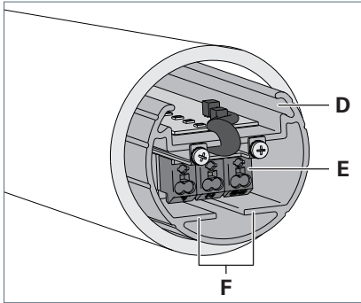
Fig. 9: Mounting profile and terminal.
